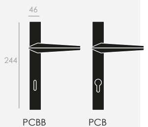
PLACA RECTANGULAR RECTANGULAR BACKPLATE
